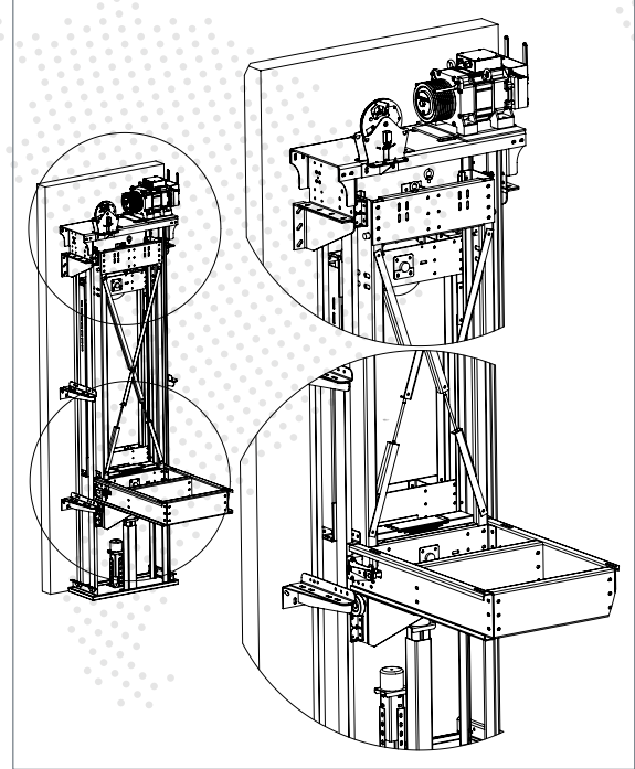
MRL L Karkas Machine roomless L frame
