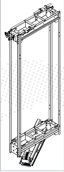
MRL Altan - Çapraz Palanga Machine roomless underslung cross type pulley system
