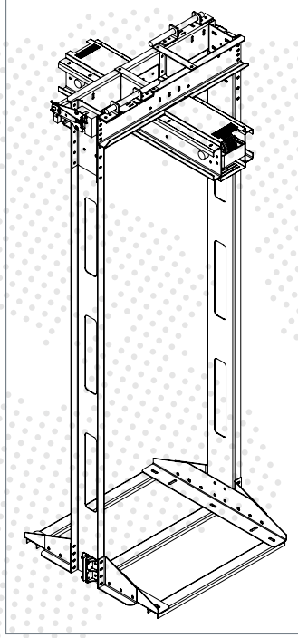
T Planga - Kuyu Dibi T type pulley at pit
