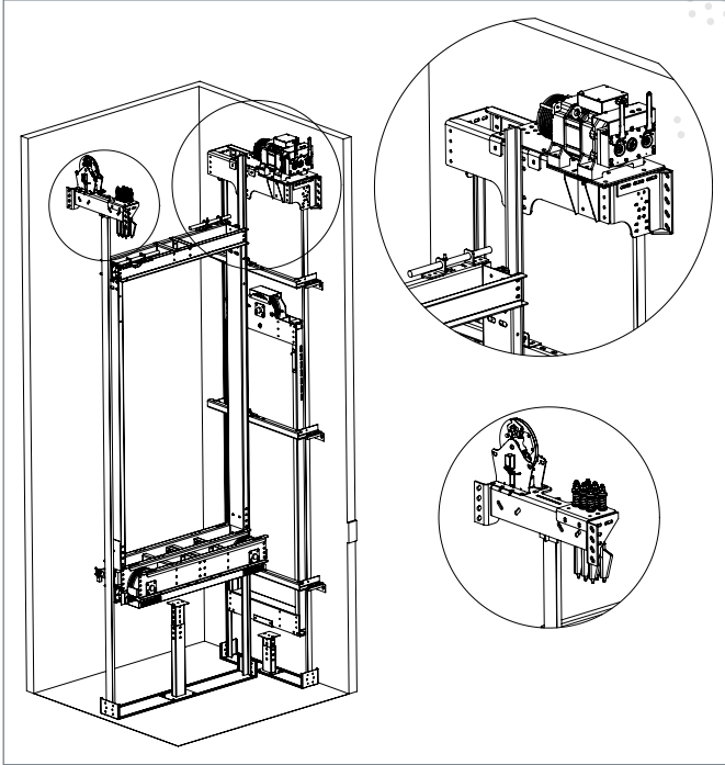
MRL Yandan Ağırlık Machine roomless elevator with side weight
